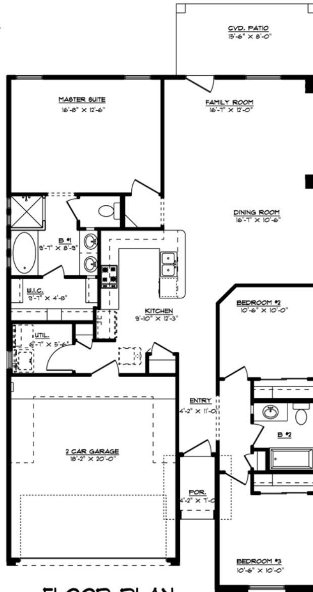
FLOOR PLAN
