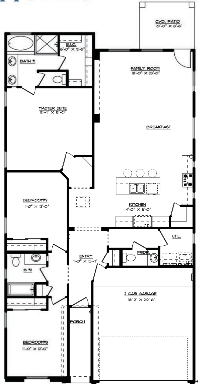
FLOOR PLAN
